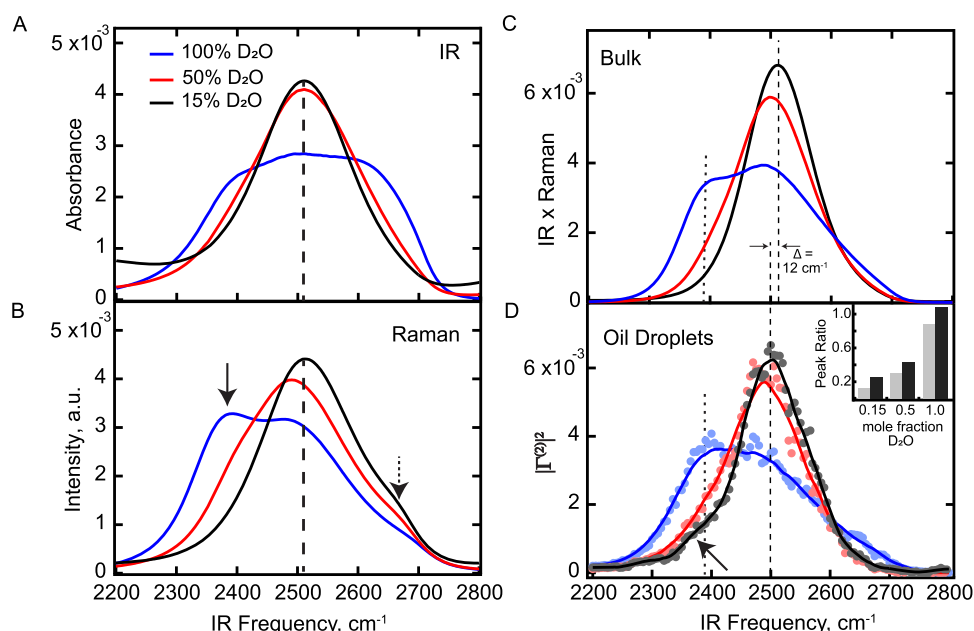
Figure 2. Isotopic dilution and the vibrational spectra of bulk and nanodroplet interfacial \text{D}_2\text{O} . (A) IR and (B) vertically polarized Raman spectra of different \text{D}_2\text{O}/\text{H}_2\text{O} mixtures containing 100 vol % \text{D}_2\text{O} (blue), 50 vol % \text{D}_2\text{O} (red), and 15 vol % \text{D}_2\text{O} (black). (C) Product of the vertically polarized Raman spectrum with the IR spectrum for different isotopic dilution ratios. (D) |\Gamma^{(2)}|^2 spectrum of oil droplets dispersed in \text{D}_2\text{O}/\text{H}_2\text{O} mixtures recorded using the SSP polarization combination. The solid lines represent the running average and are a guide to the eye. The vertical dashed line represents the peak frequency of the uncoupled O–D mode as seen in the spectrum of 15% \text{D}_2\text{O} . The vertical dotted lines indicate the presence of a strongly H-bonded O–D population at the oil droplet surface compared to bulk. The legends correspond to volume % of \text{D}_2\text{O} added in the mixture. The inset shows the 2395/2500 \text{cm}^{-1} peak ratio from the oil droplets (black) and bulk water (gray) at different \text{D}_2\text{O}/\text{H}_2\text{O} ratios. Note that all spectra are normalized to their area.
